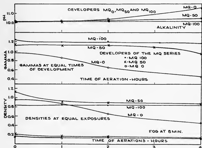
FIG. 5. Effect of aeration of developers containing various proportions of elon and hydroquinone.
